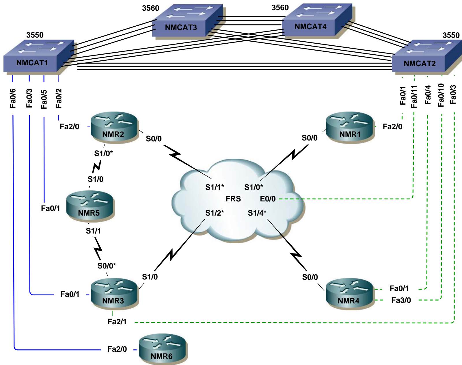
NMC-DoITv6 Lab Diagram Rack Two – Revision I CCIErack.com
